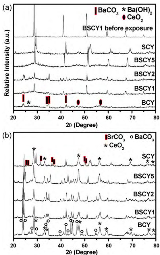
Fig. 5. (a) XRD patterns of the sintered BSCY pellets after exposure in boiling water for 4 h and (b) XRD patterns of the sintered BSCY pellets after exposure in wet \text{CO}_2 at 700^\circ\text{C} for 12 h.
